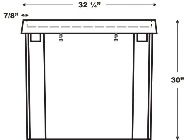
END VIEW
